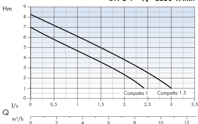
DN G 1" 1/4 - 2850 1/min
